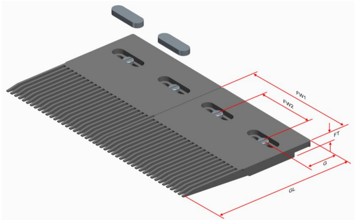
Finger Transfer Plate Frame Dimensions
